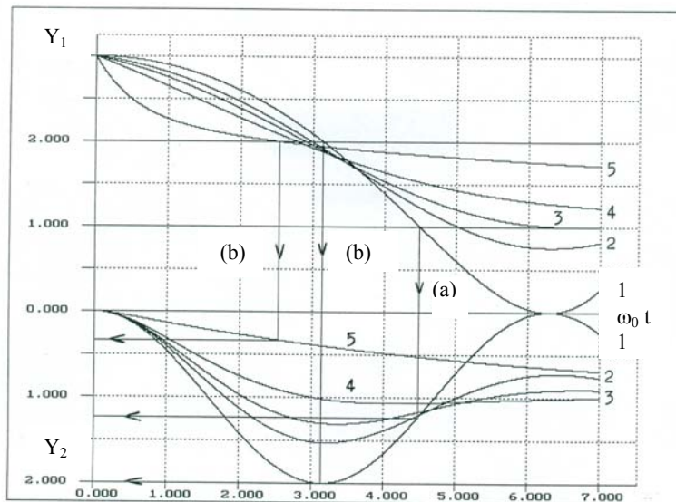
Fig. 1. The curves Y_1(t \cdot \omega_0) and Y_2(t \cdot \omega_0) for transfer function (15) and five values of B = 0, 0.2, 0.35, 0.65, 3 . The bigger B the bigger the digit indicating the respective curve.
