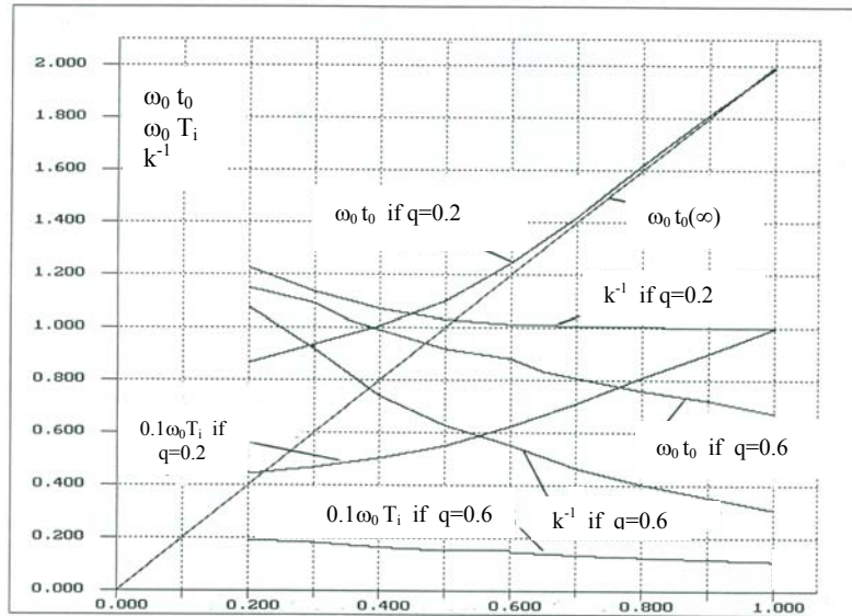
Fig. 2. The curves \omega_0 t_0(B), \omega_0 t_0(\infty), 0.1 T_i(B) \omega_0 t_0(B), and k^{-1}(B) obtained for q equal to 0.2 and 0.6.
