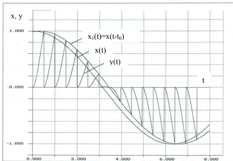
Fig. 3. The input signal x(t) = \cos 0.5t , the perfectly delayed input signal x_1(t_0) and the output signal y(t) of an expanding system based on transducer (15) with B = 3 .
